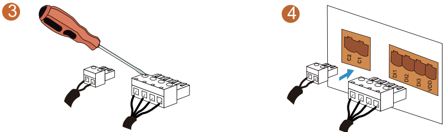
The following figure shows the cable connection between the box and the inverter.
