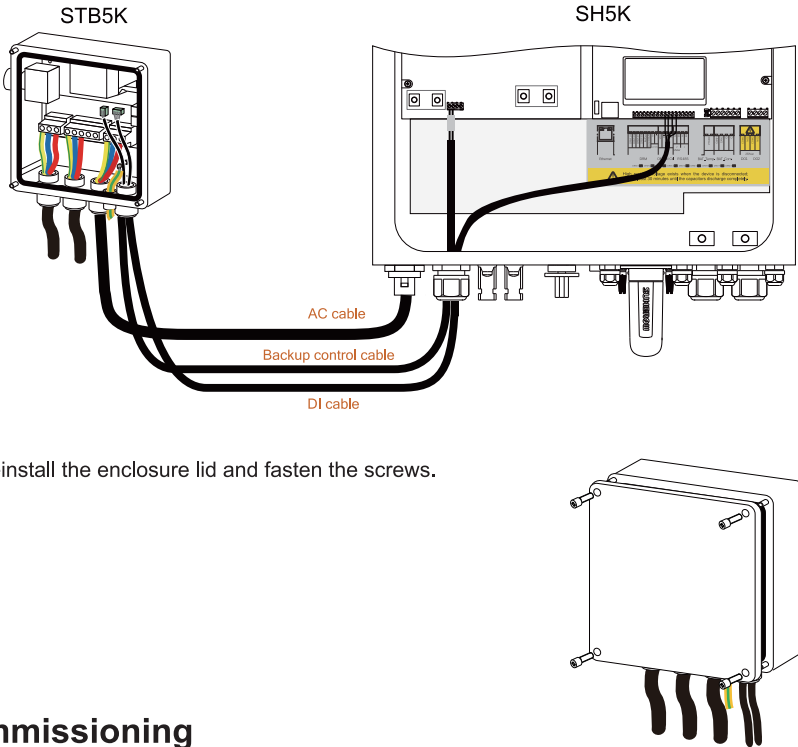
The following figure shows the cable connection between the box and the inverter.
